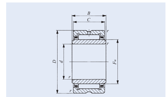
Fig. 7 Machined Type Needle Roller Bearing
