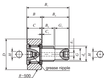
CFKRE ... R Outside diameter of eccentric collar d_e 13mm
