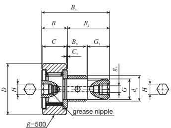
CFKRE ... R Outside diameter of eccentric collar d_e 15~35mm
