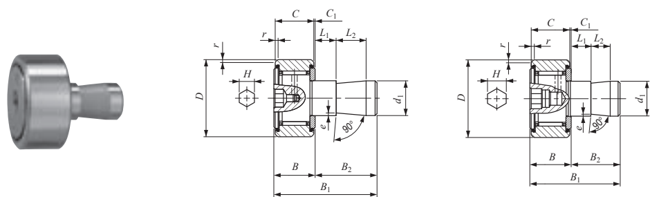
CF-SFU...B Stud dia. d_1 6-10mm CF-SFU...B Stud dia. d_1 12-20mm
