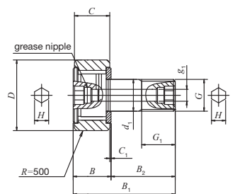
CFKR...VR Outside dia. of outer ring D 22, 26 mm
