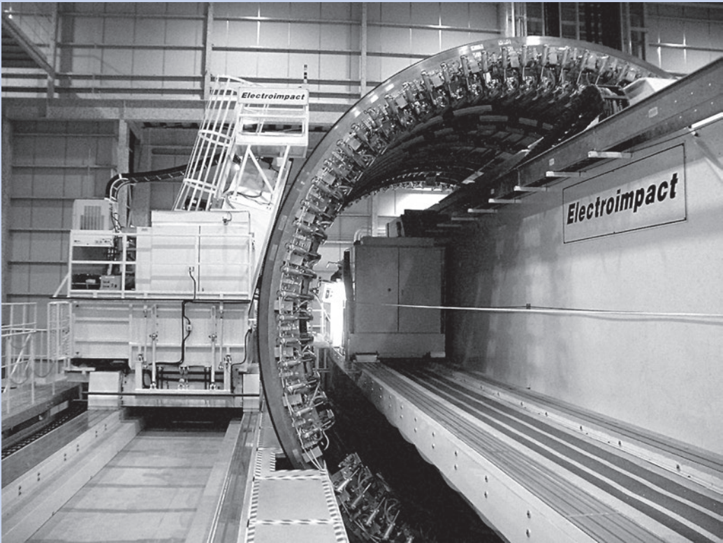
Locating machines for airplane body panels
